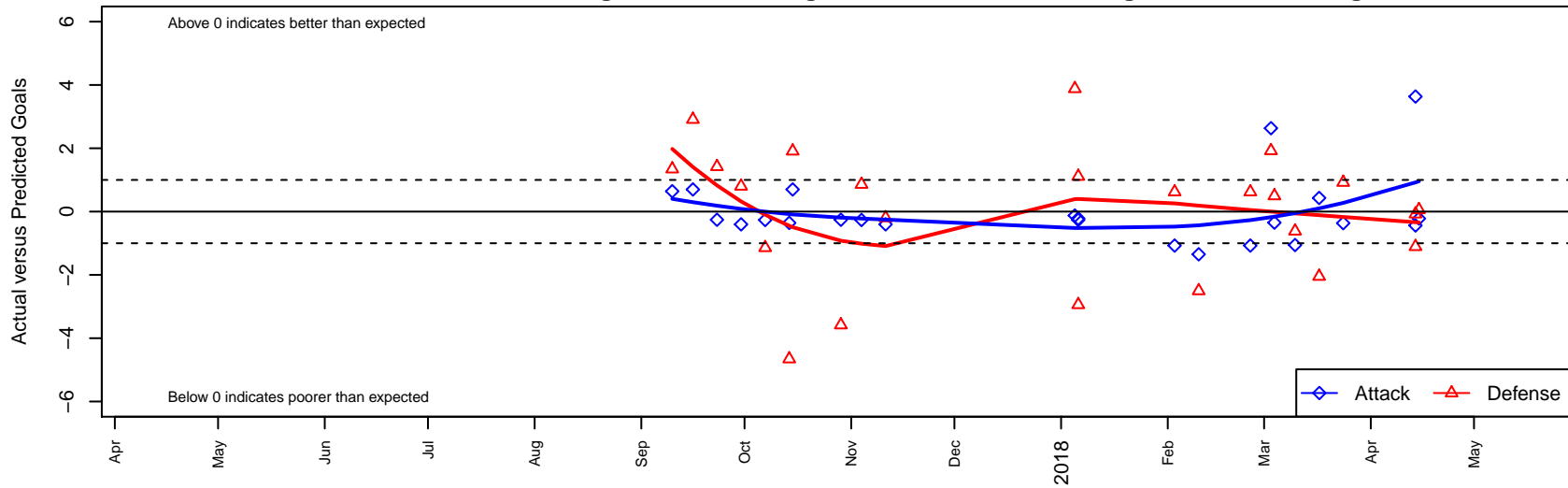
FC Bellevue G04 Dots are actual minus expected GF (blue circles) and GA (red triangles). Blue line is smoothed change in attack strength. Red is smoothed change in defense strength.
